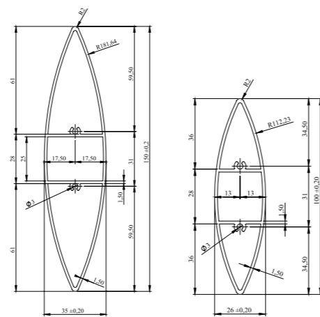
Type 1 Section
